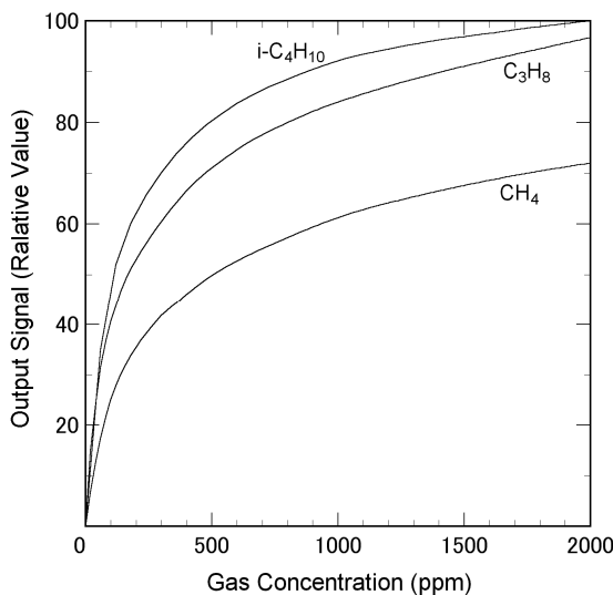
Fig 1 Sensitivity characteristic
