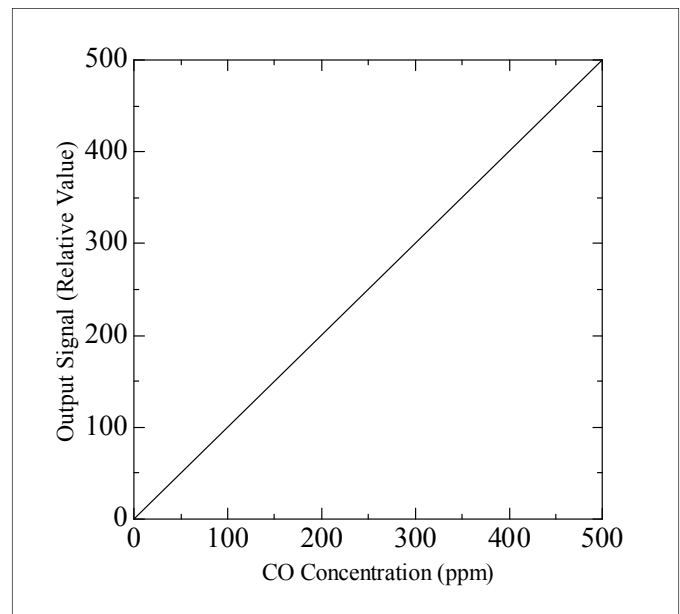
Fig. 2 Sensitivity characteristic
