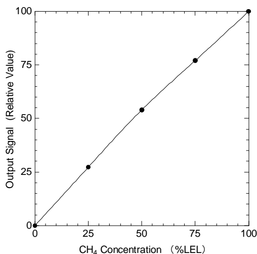
Fig 1 Sensitivity characteristic
