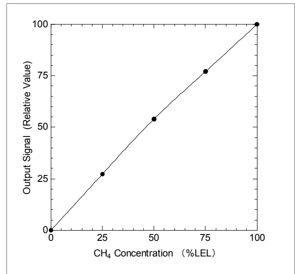
Fig 1 Sensitivity characteristic
